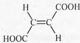
Fumaric acid
