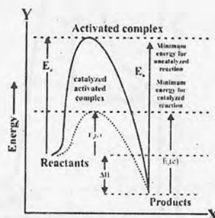
Catalyzed and uncatalyzed reaction
